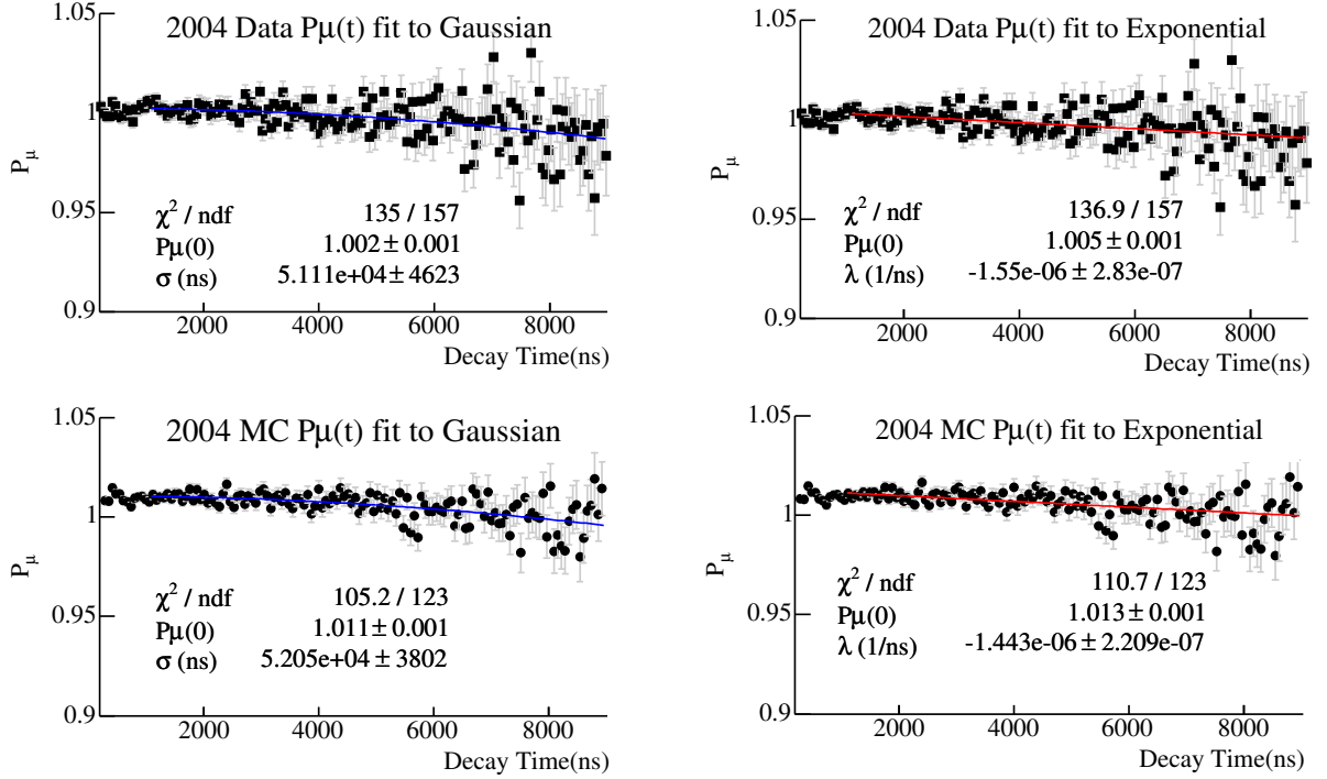
Figure 6.7: Polarization estimate from an asymmetry analysis of the 2004 data at the top, and 2004 simulation at the bottom. The distributions are fit to a Gaussian on the left and to an exponential on the right. The fit excludes decay positrons before a decay time of 1050 ns to avoid the potential bias from extra muon hits in the upstream decay positrons.
