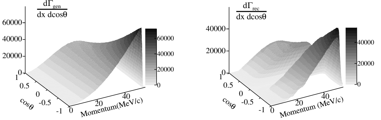
Figure 1.2: The theoretical distribution of positron angles and momenta with 100 % acceptance is shown on the left. Positrons that pass the TWIST detector acceptance have the distribution shown on the right.
