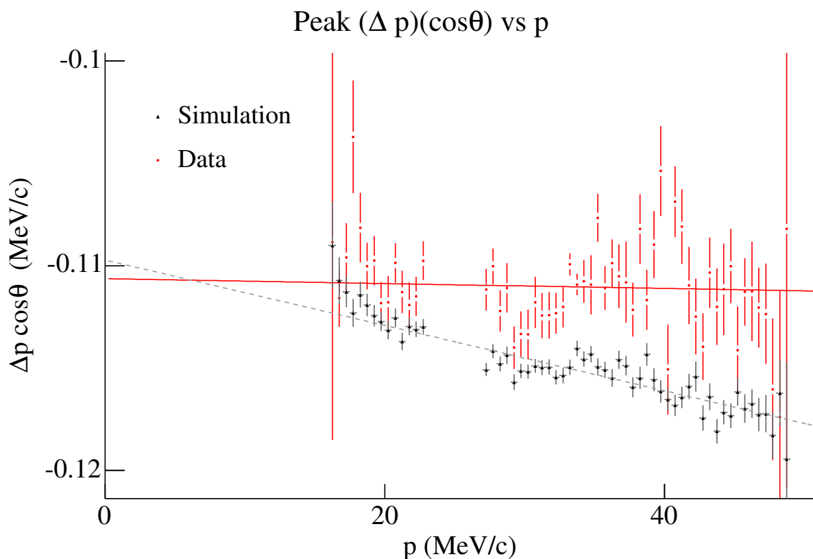
Figure 6.11: Comparison of \Delta p \cos \theta versus p in Data and simulation. \Delta p comes from the difference in upstream and downstream fits to positrons from a data set with muon stopping upstream in the trigger scintillator and PCs.
