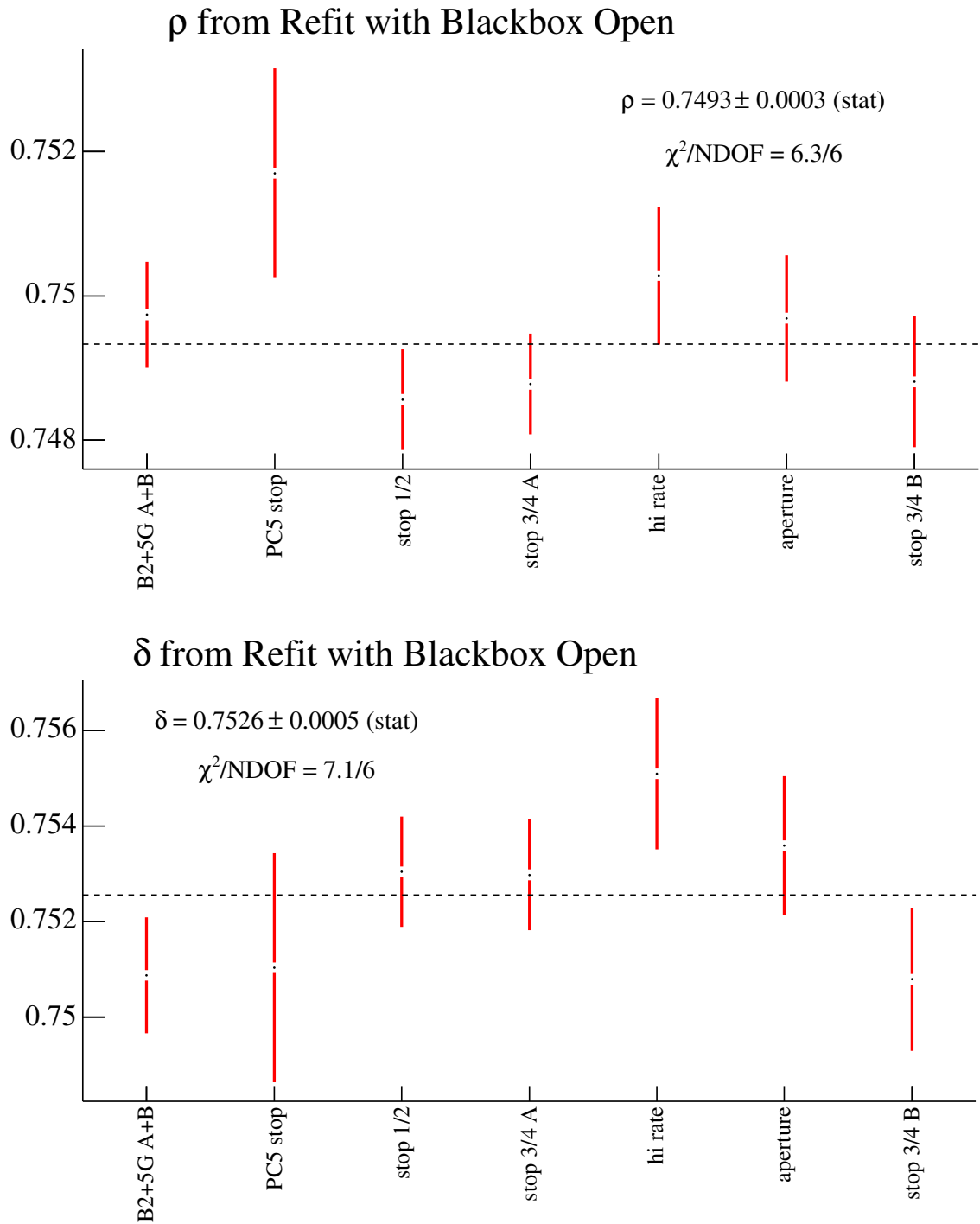
Figure 7.6: The values of \rho are shown in the top plot, and the values for \delta are shown in the bottom plot. Only the statistical uncertainty is shown, because the measurements of \rho and \delta have not been completed.
