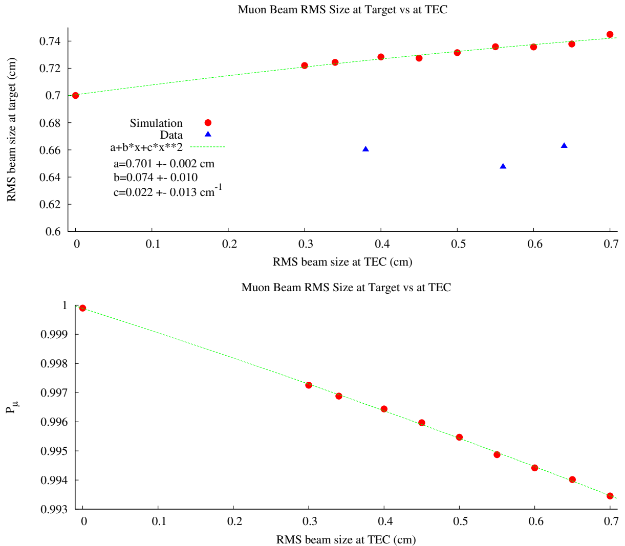
Figure 6.4: The top plot shows the muon beam size at the stopping target versus at the TEC, where the simulation points are solid circles and the data points are solid triangles. The bottom plot shows the muon polarization predicted by the simulation for different muon beam sizes at the TEC.
