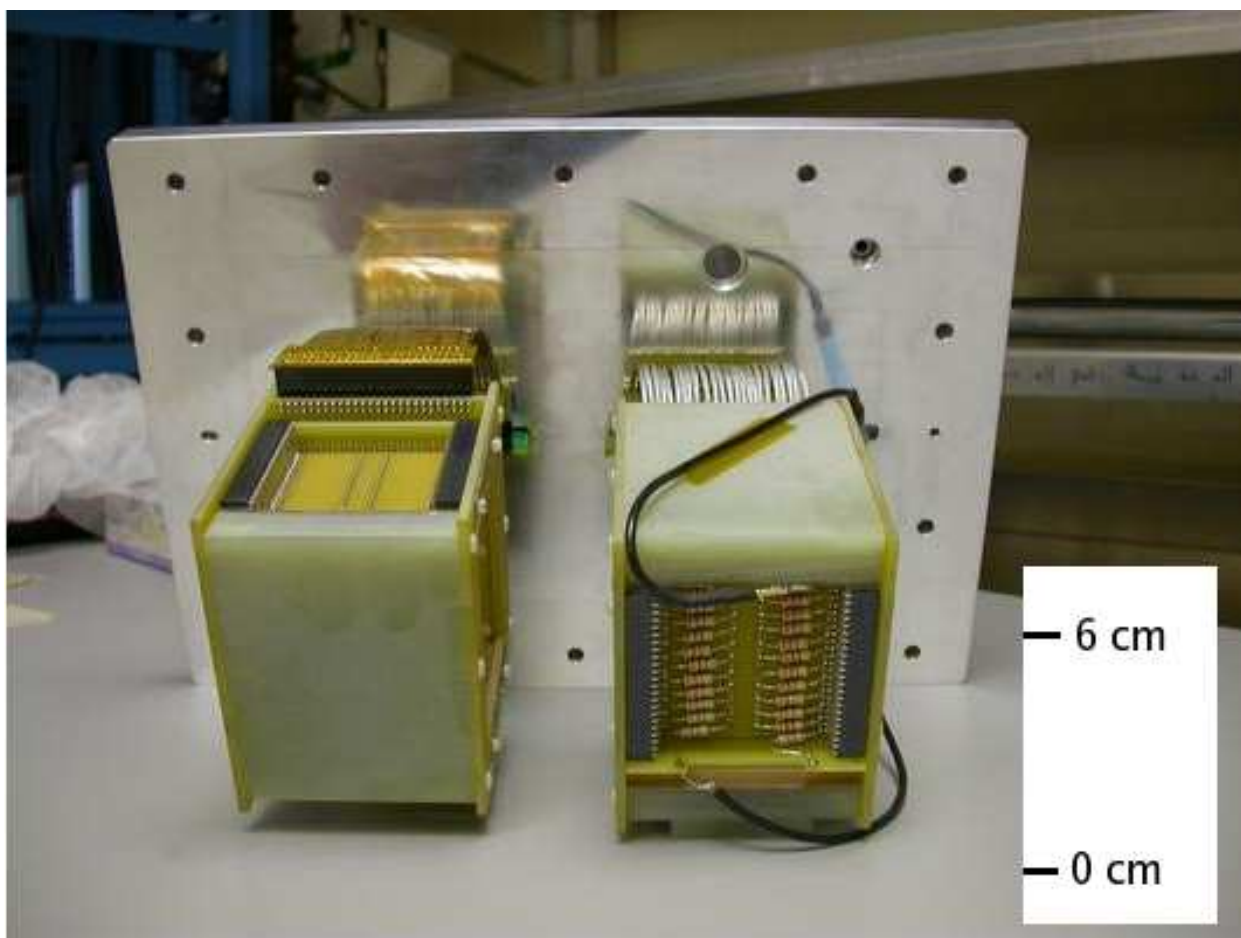
Figure 2.14: Photograph showing the TEC modules and mounting lid removed from the TEC box.
