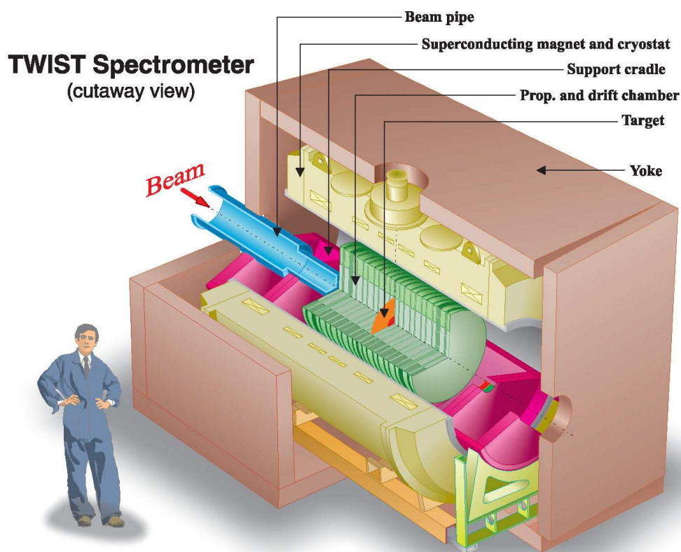
Figure 2.5: The TWIST spectrometer. (Courtesy of TWIST .)
