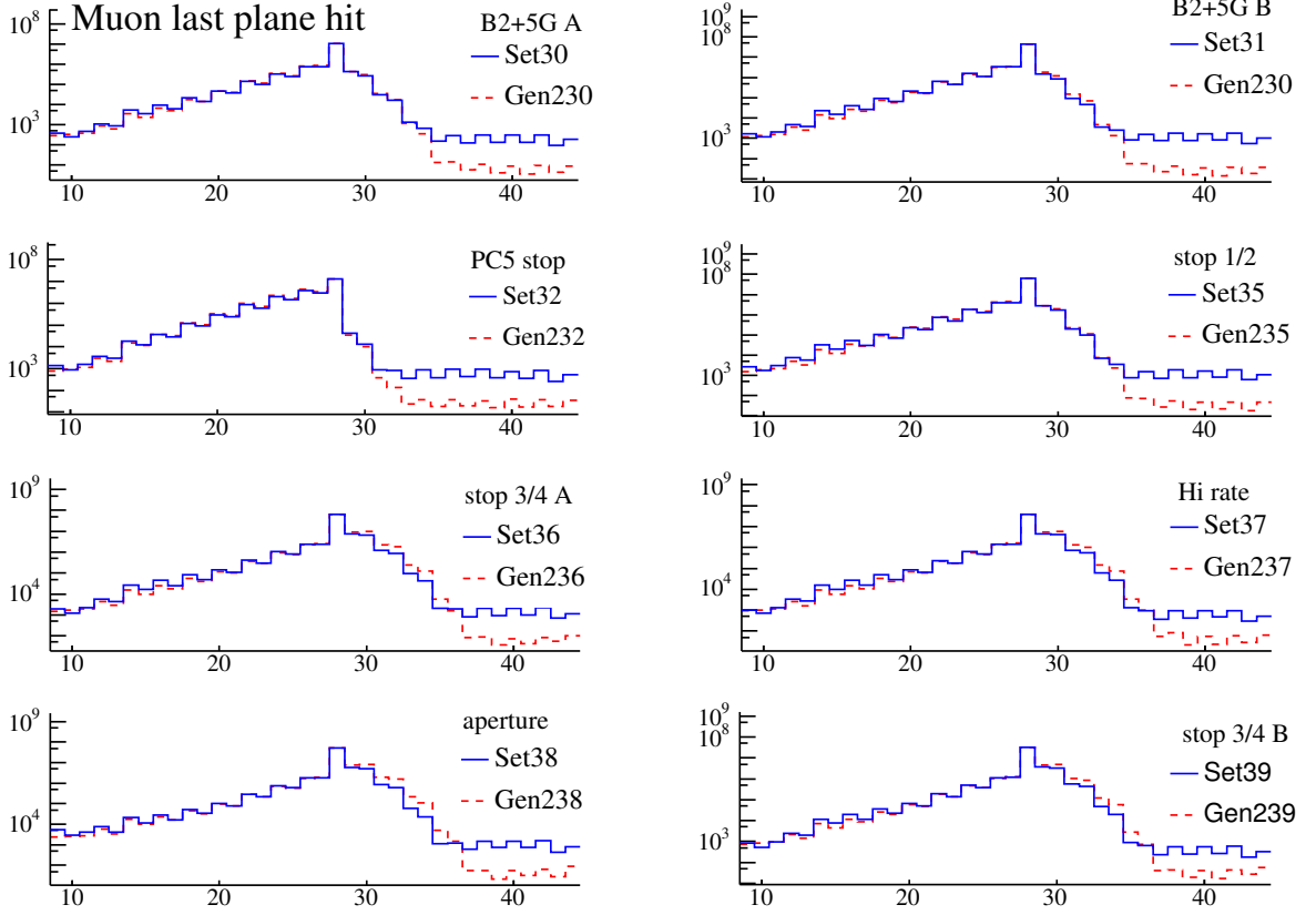
Figure 4.3: Overlay of the muon stopping distribution as a function of last plane number hit, where the MC is in red and the data is in blue.
