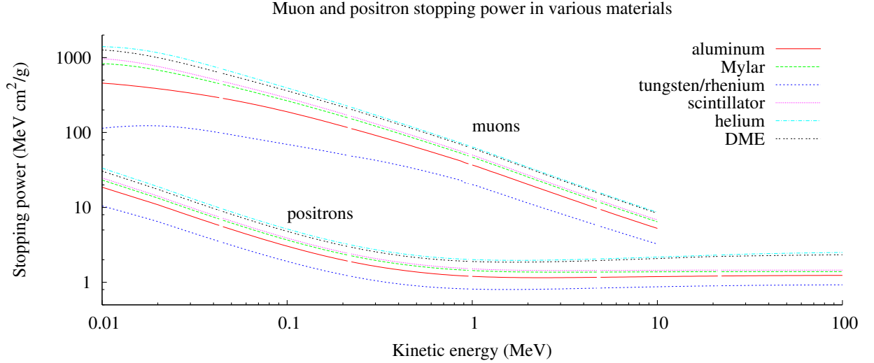
Figure 1.5: Stopping power of positrons and muons in several materials for the range of energies tracked in the simulation. Below the lowest energy on this plot, the stopping power for muons drops again and can be estimated using the Lindhard model.
