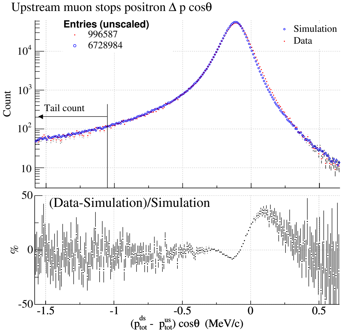
Figure 5.3: Energy losses, from an analysis of the decay positrons from far upstream muon stops, in data and simulation, are overlaid in the top plot, and shown as a percent difference in the bottom plot.
