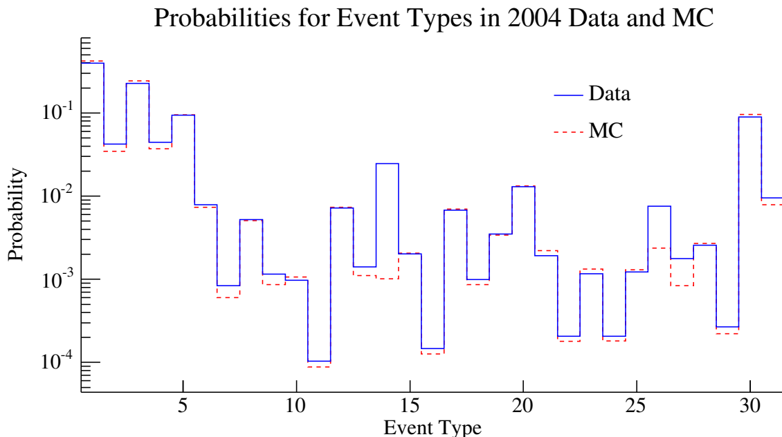
Figure 3.2: Distribution of event types in 2004 data and simulation. Event type 14 is the beam positron trigger events that should only occur in the data. The beam positron trigger classifications of the simulation occur for beam positrons that come close in time to a muon.
