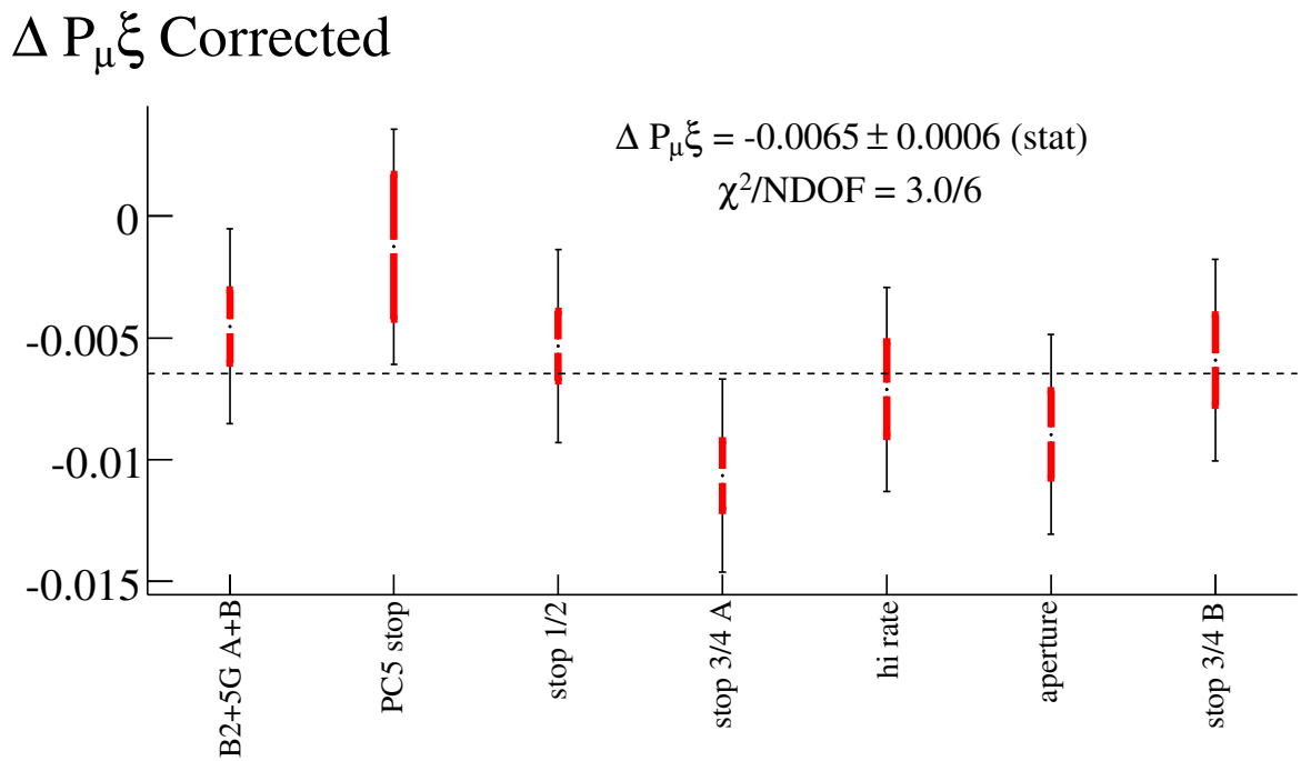
Figure 7.3: \Delta P_{\mu\xi} from 2004 data to simulation fits, with all of the required corrections applied. The thick red error bars are statistical only, and the longer thin black error bars include the set to set systematic uncertainty added in quadrature with the statistical uncertainty.
