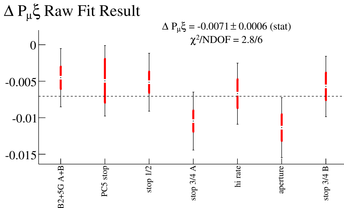
Figure 7.2: \Delta P_\mu \xi from 2004 data to simulation fits, with simulation fringe field of production running.
